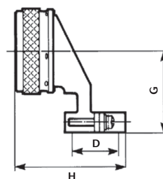
Elbow cable clamp Type 51 (aluminum)
